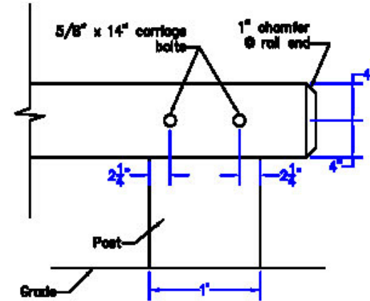
FRONT ELEVATION nbs
