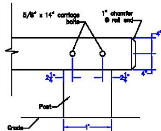
FRONT ELEVATION nta
