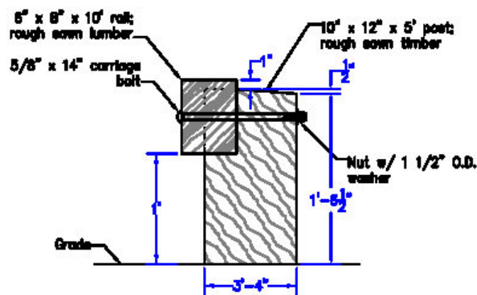
SECTION nta
