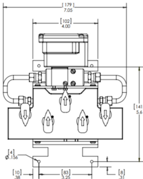
Figure 6-6. Transducer with 5-port Manifold
