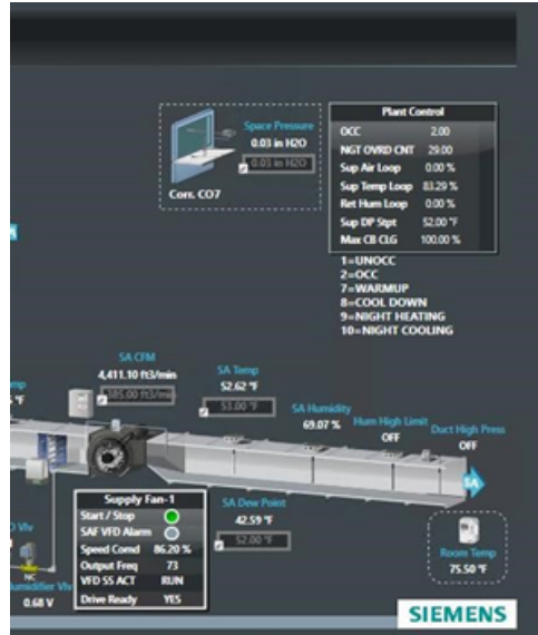
Figure 6-4. System Mode Points and Key Performance Indicators
