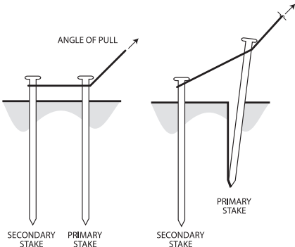
Figure 17. Double Staking
