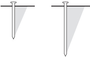
Figure 11. Soil Wedge (Bulb) Size and Sideways Resistance
